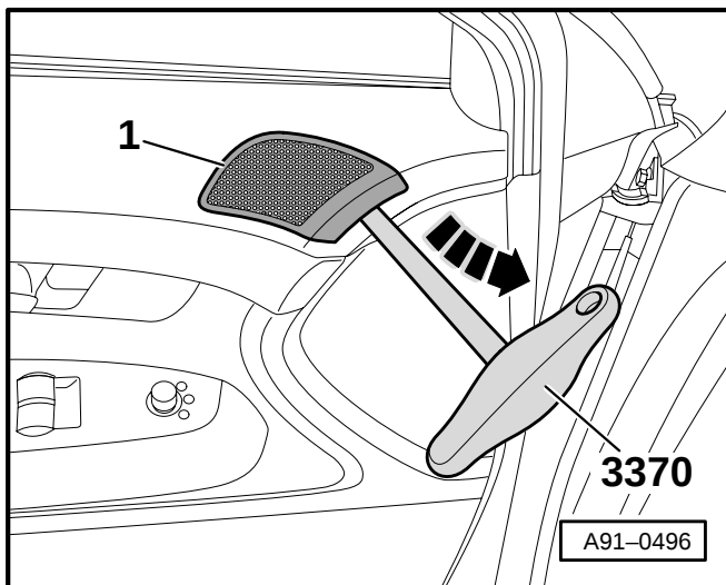
Fig. 11 Mid-range/treble loudspeakers, front
