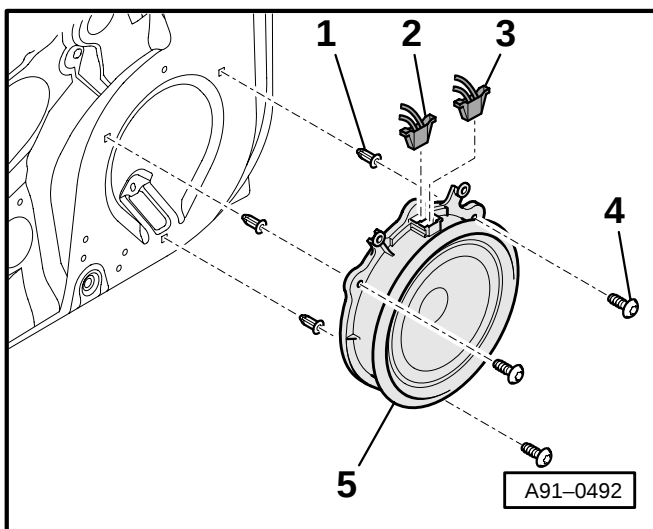
Fig. 12 Bass loudspeakers, front
