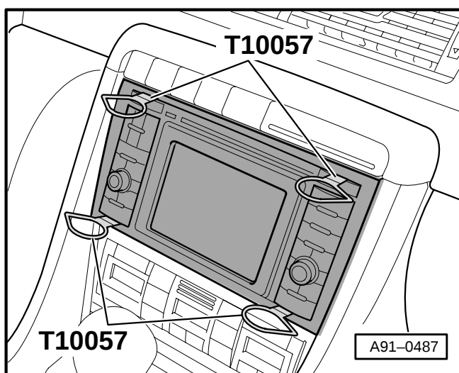
Fig. 2 Operating electronics control unit, navigation - J402
