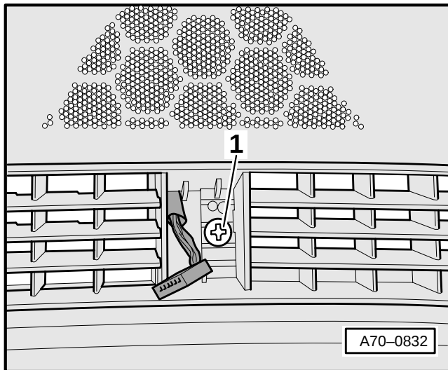
Fig. 13 Internal loudspeaker (centre loudspeaker) - R70
