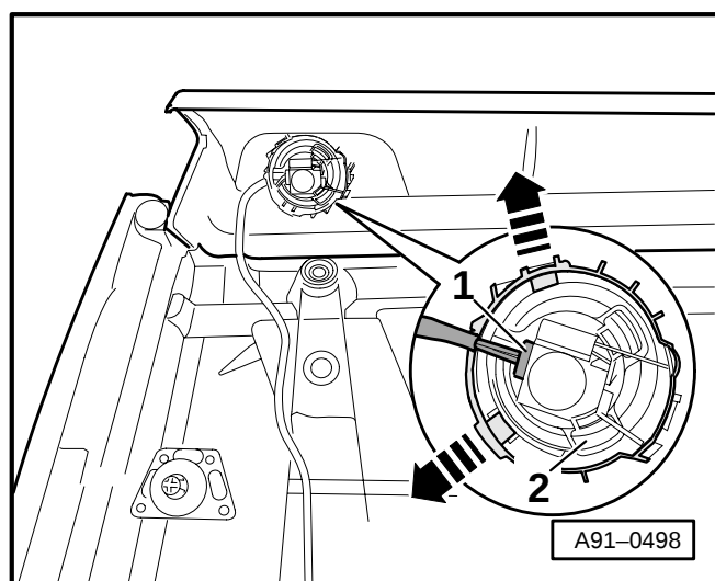
Fig. 9 Mid-range/treble loudspeakers, rear
