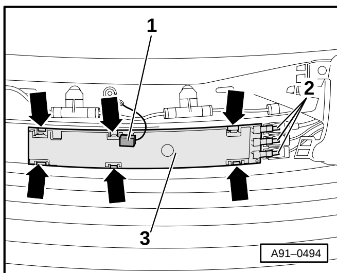
Fig. 5 Aerial amplifier or aerial selection control unit - J515
