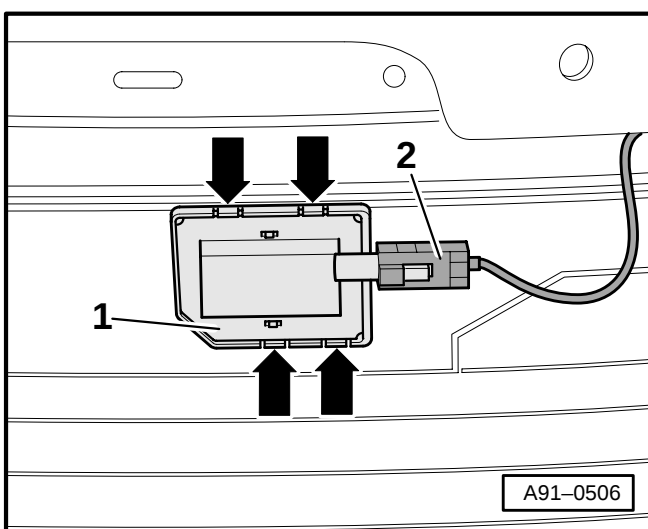
Fig. 3 Navigation aerial (GPS) - R50
