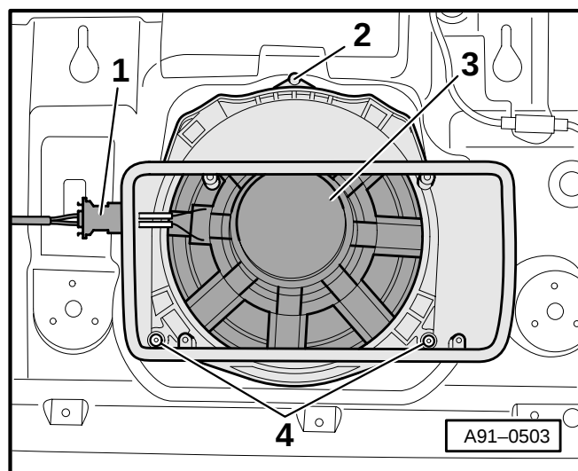
Fig. 8 Bass loudspeaker (subwoofer) - R100
