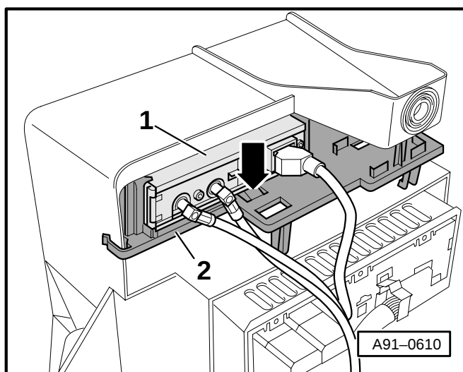
Fig. 6 Navigation interface - R94
