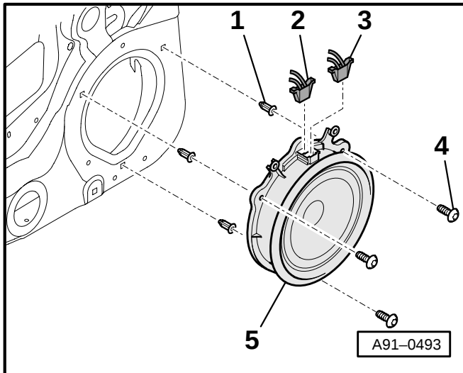
Fig. 10 Bass loudspeakers, rear
